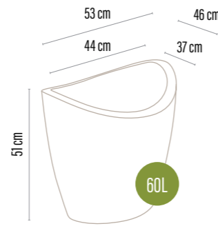
ALYG-14 GONDOL POT NO.2 Gondol Saksı No.2 44 x 53 x 51 cm Ø37 x 46 cm 0,1189 m 3 2750 g
